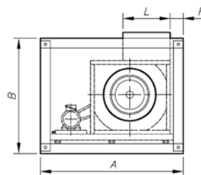
Vertical impulsion on request (V) LG-90
