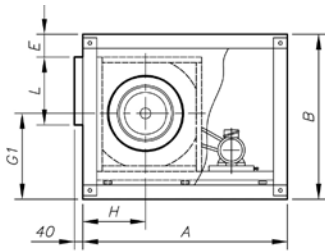
Standard supply horizontal impulsion (H) RD-90
