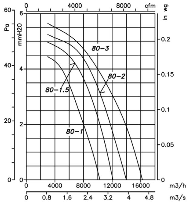
12 poles (2-speed 6/12 motor)
