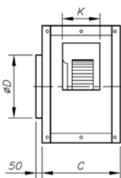
Horizontal impulsion on request (H) LG-90
